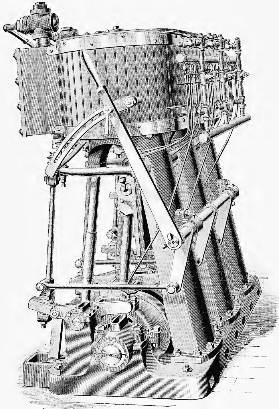
THE DAVIS-FARRAR TRIPLE-EXPANSION YACHT ENGINE.
